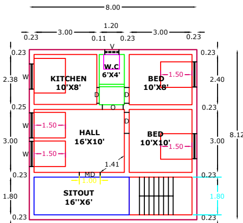
GROUND FLOOR RESIDENTIAL PLAN
