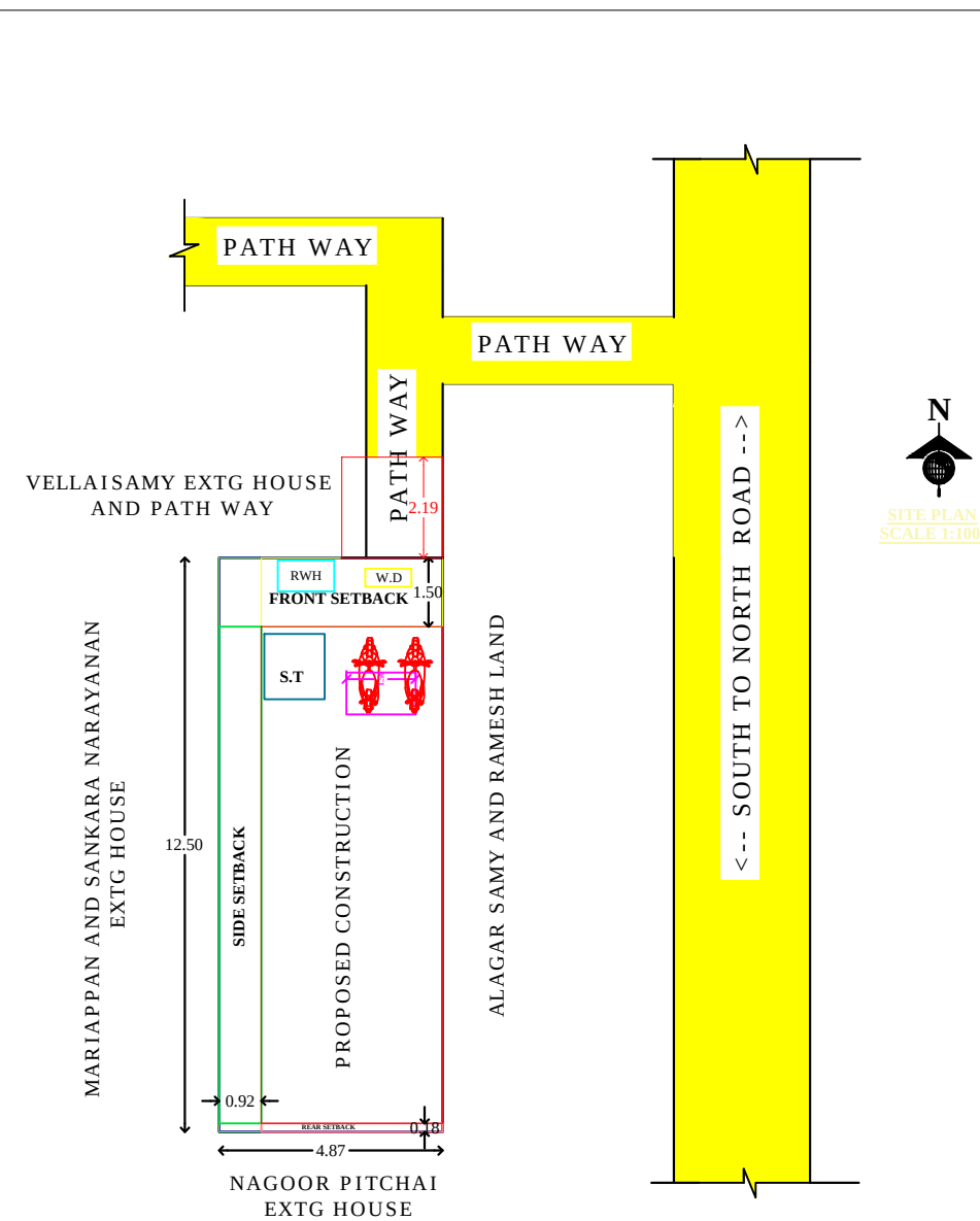
SITE PLAN
