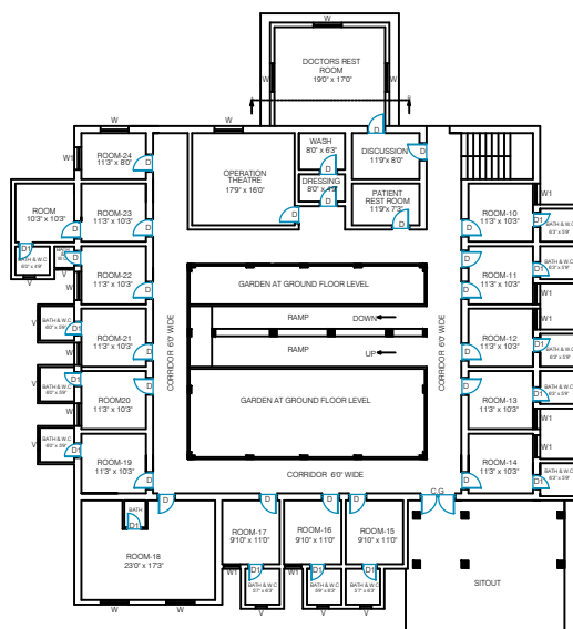
EXG.FIRST FLOOR PLAN
