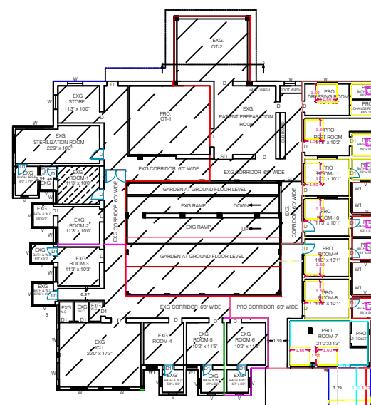
EXG & PRO SECOND FLOOR PLAN
