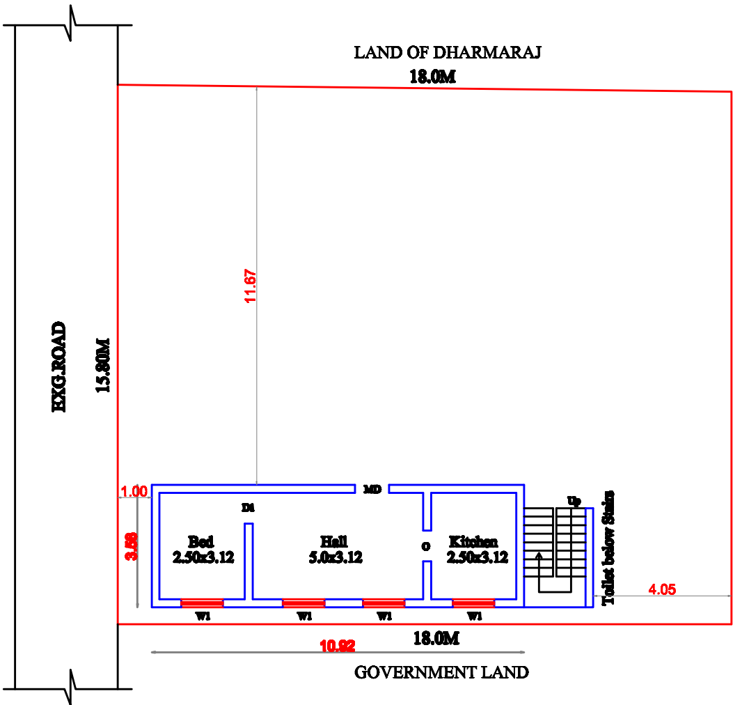
PRO.SITE CUM GROUND FLOOR PLAN
