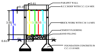
SECTION ON "AA"
