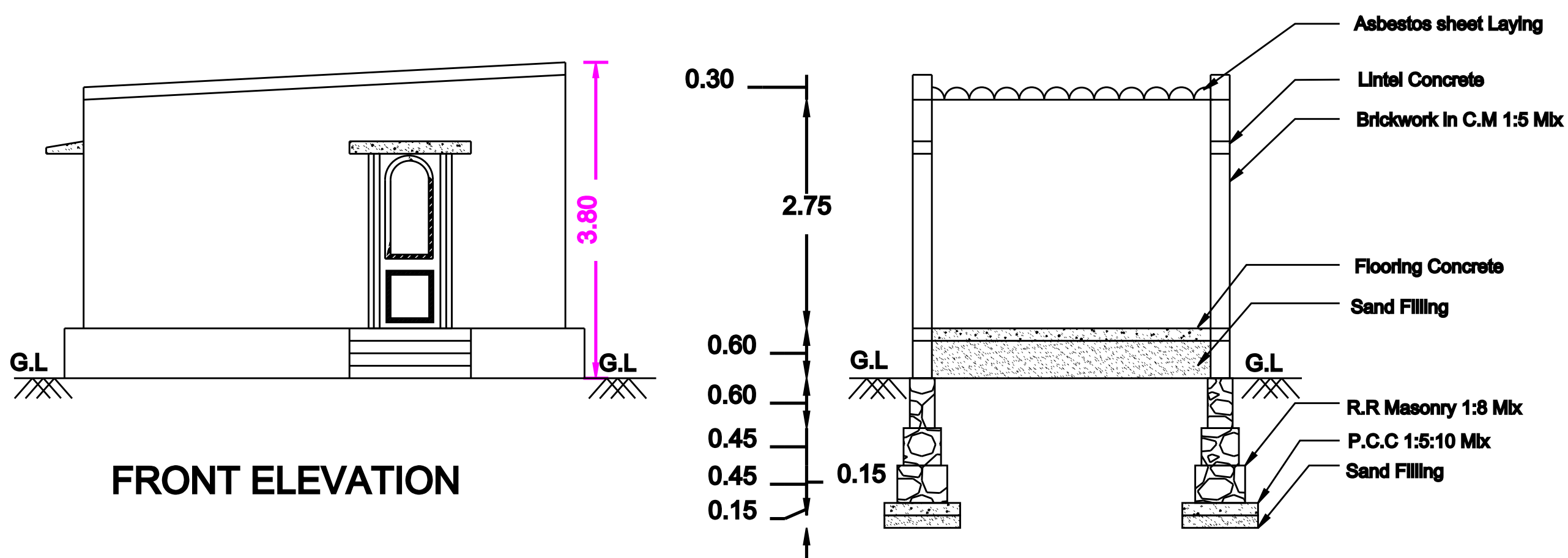
SECTION ON SS
