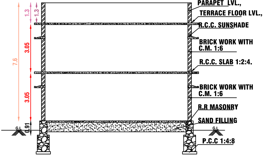
SECTION ON A-A & A'-A'
