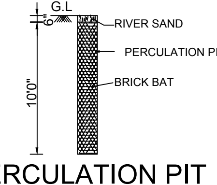
PERCOLATION PIT
