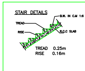
STAIR DETAILS
