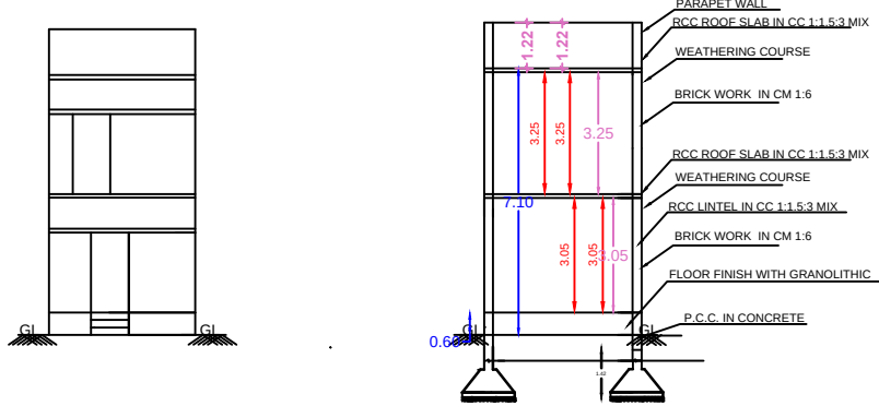
ELEVATION SECTION ON AA
