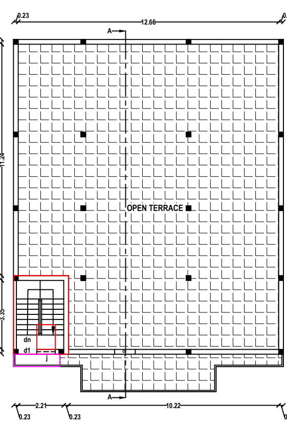
PLAN - HEAD ROOM PROPOSED - RESIDENCE
