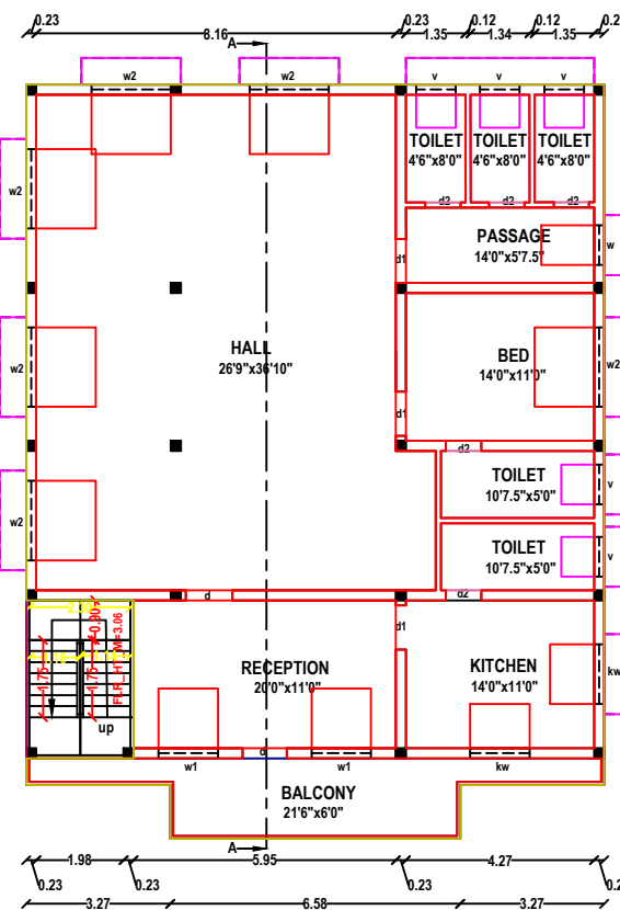
PLAN - FIRST FLOOR PROPOSED - RESIDENCE
