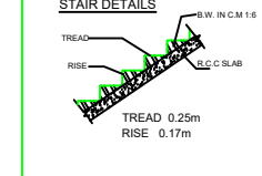
STAIR DETAILS
