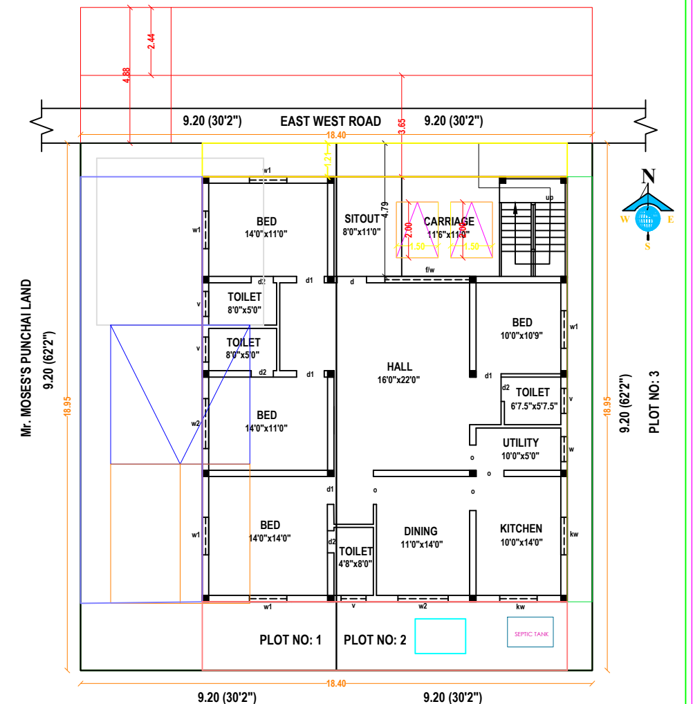
SITE PLAN SCALE:- 1:100 Mr. GEORGE VARGEE'S PUNCHAI LAND
