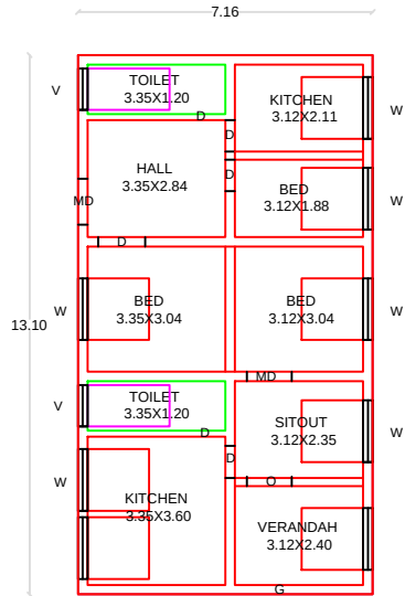
PROPOSED FF PLAN
