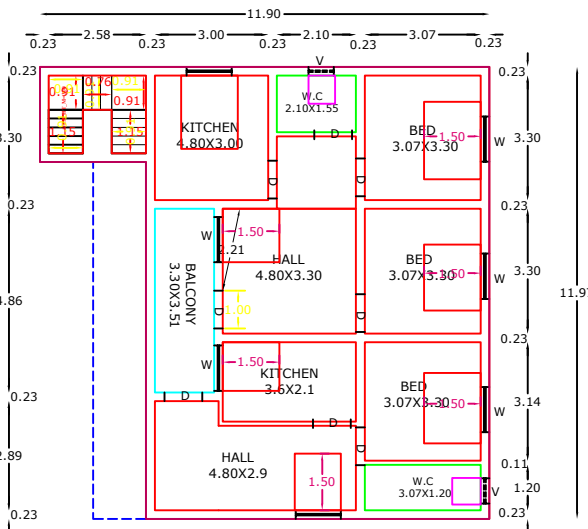
PRO FIRST FLOOR RESIDENTIAL PLAN
