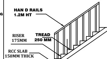
STAIRCASE DETAILS SCALE 1:50
