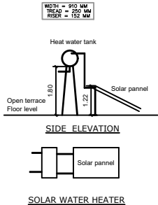
SOLAR WATER HEATER
