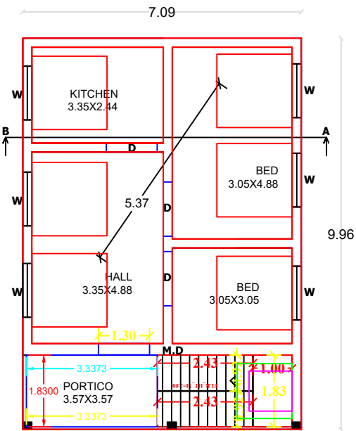
PLAN
