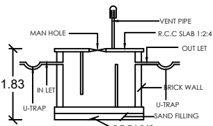
SECTION E.F. SEPTIC TANK DETAIL
