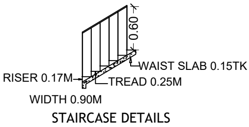
STAIRCASE DETAILS
