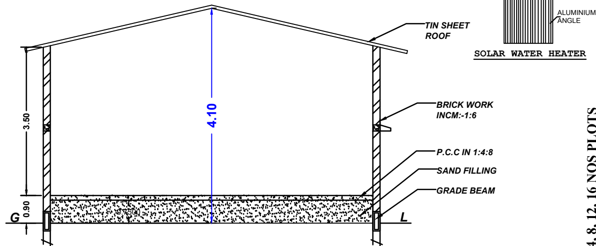
SECTION "AB"
