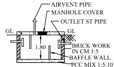
SECTION ON SEPTICTANK
