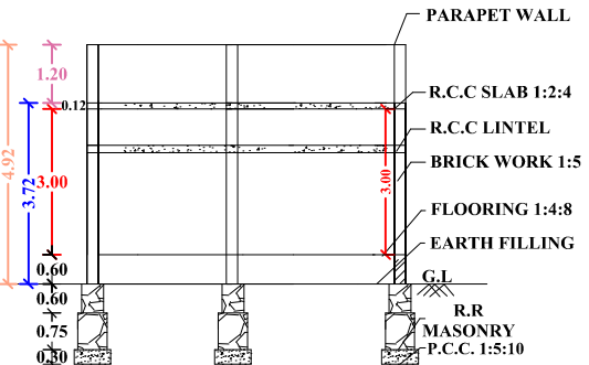
"SECTION "AB"
