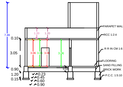
SECTION AB
