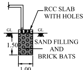
SECTION OF BS
