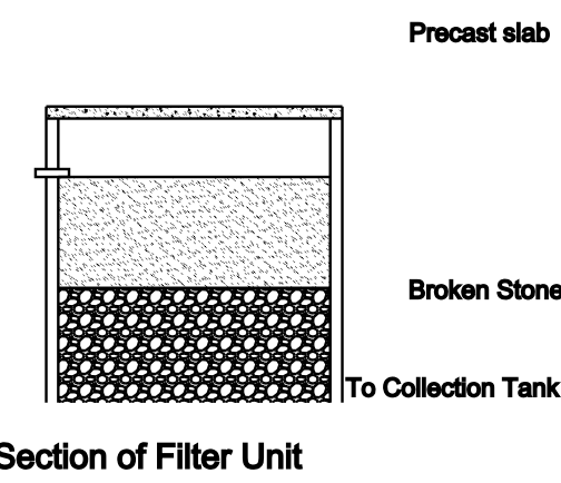
Section of Filter Unit
