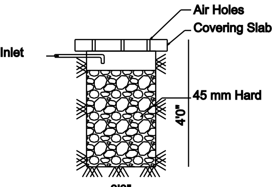
Rain Water Perculation Pit (Not to Scale)
