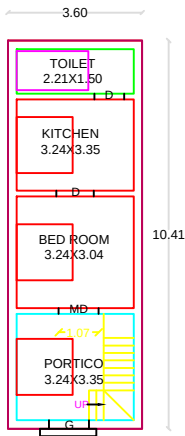
PROPOSED GF PLAN
