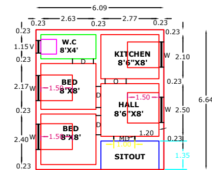
GROUND FLOOR RESIDENTIAL PLAN
