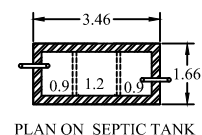
PLAN ON SEPTIC TANK
