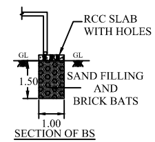
SECTION OF BS
