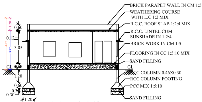
SECTION OF "BS"
