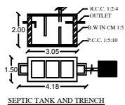
SEPTIC TANK AND TRENCH
