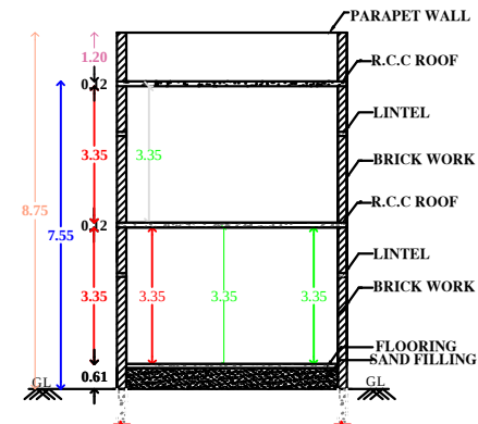
"SECTION "AB"
