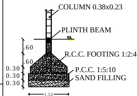
COLUMN DETAILS
