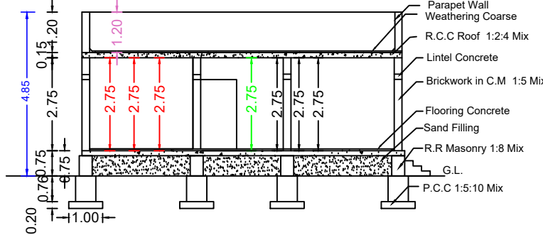
SECTION ON SS
