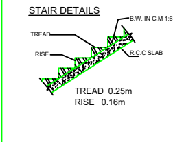
STAIR DETAILS
