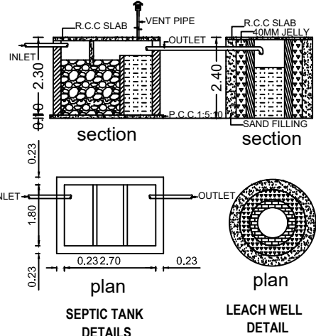
1000 GALLONS CAPACITY SEPTIC TANK (NTS)
