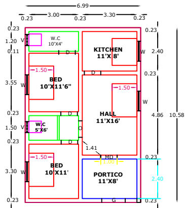
PRO GROUND FLOOR RESIDENTIAL PLAN
