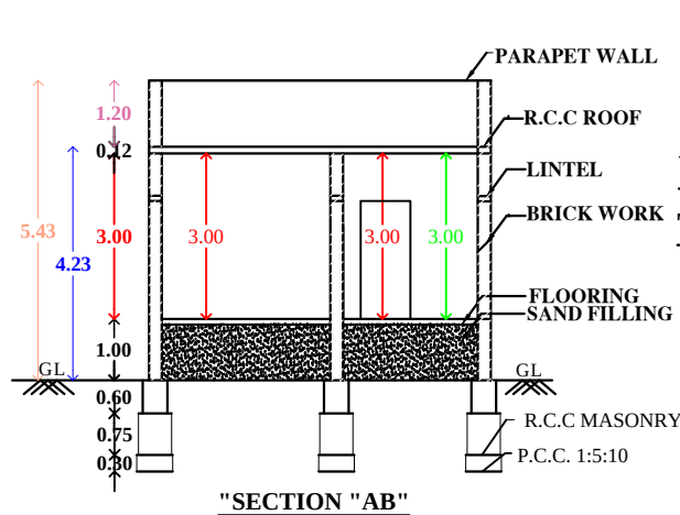
"SECTION "AB"
