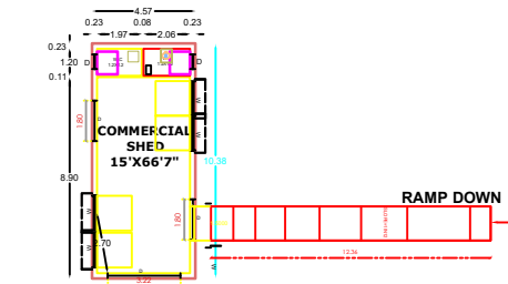
PRO GROUND FLOOR COMMERCIAL PLAN
