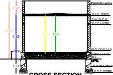
CROSS SECTION
