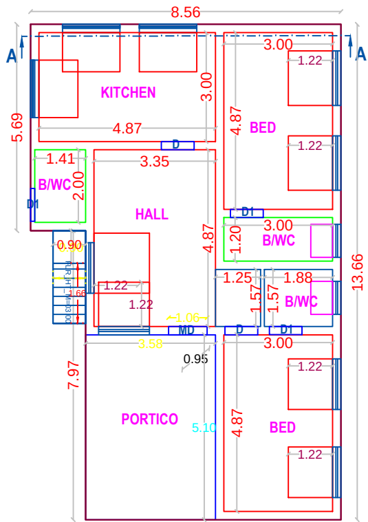
PLAN - GROUND FLOOR (PROPOSED)
