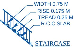
STAIRCASE
