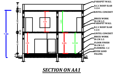
SECTION ON AA1
