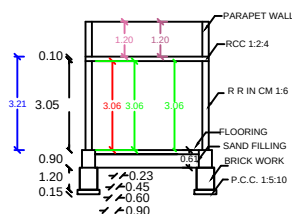
SECTION AB
