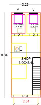
PRO SHOP GF PLAN
