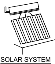
SOLAR SYSTEM
