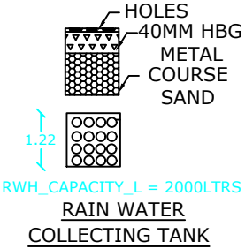
OF FILTER BED & WELL
