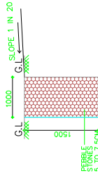
SECTION OF PEBBLE TRENCH
