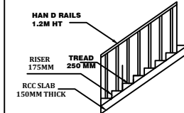
STAIRCASE DETAILS SCALE 1:50
