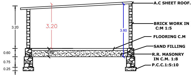
CROSS SECTION ON A-B
