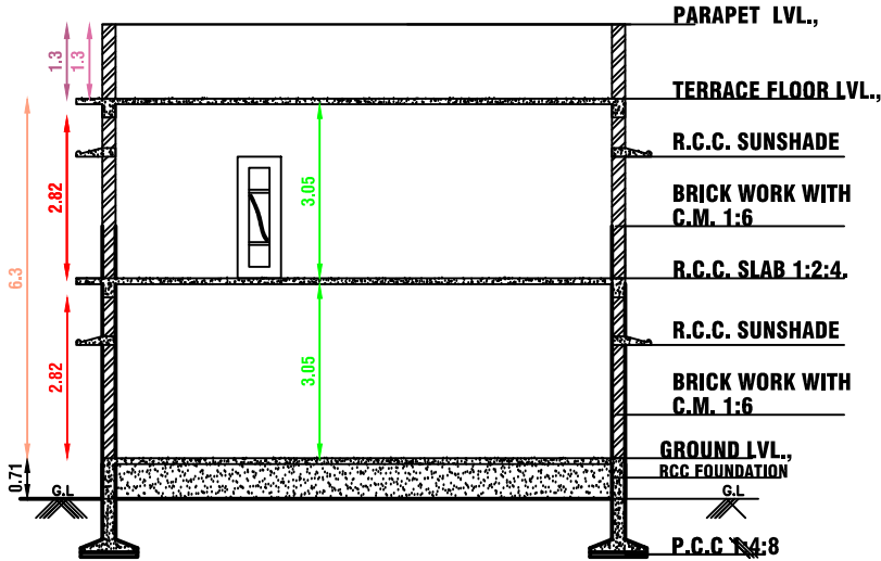
SECTION ON A-A & A'-A'
