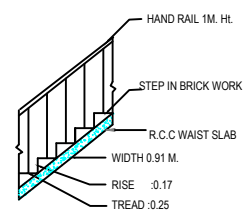
STAIR DETAIL
