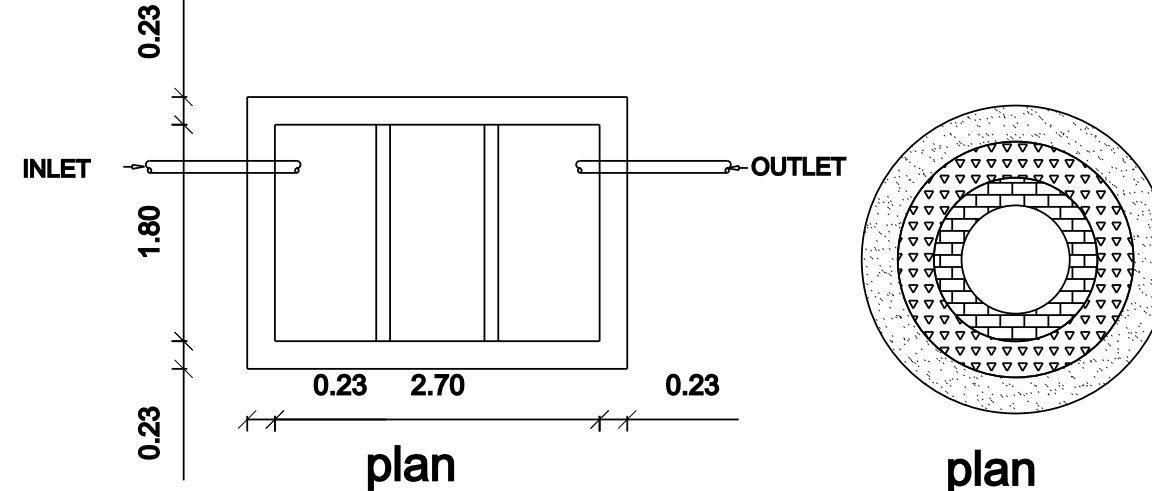
plan SEPTIC TANK DETAILS
