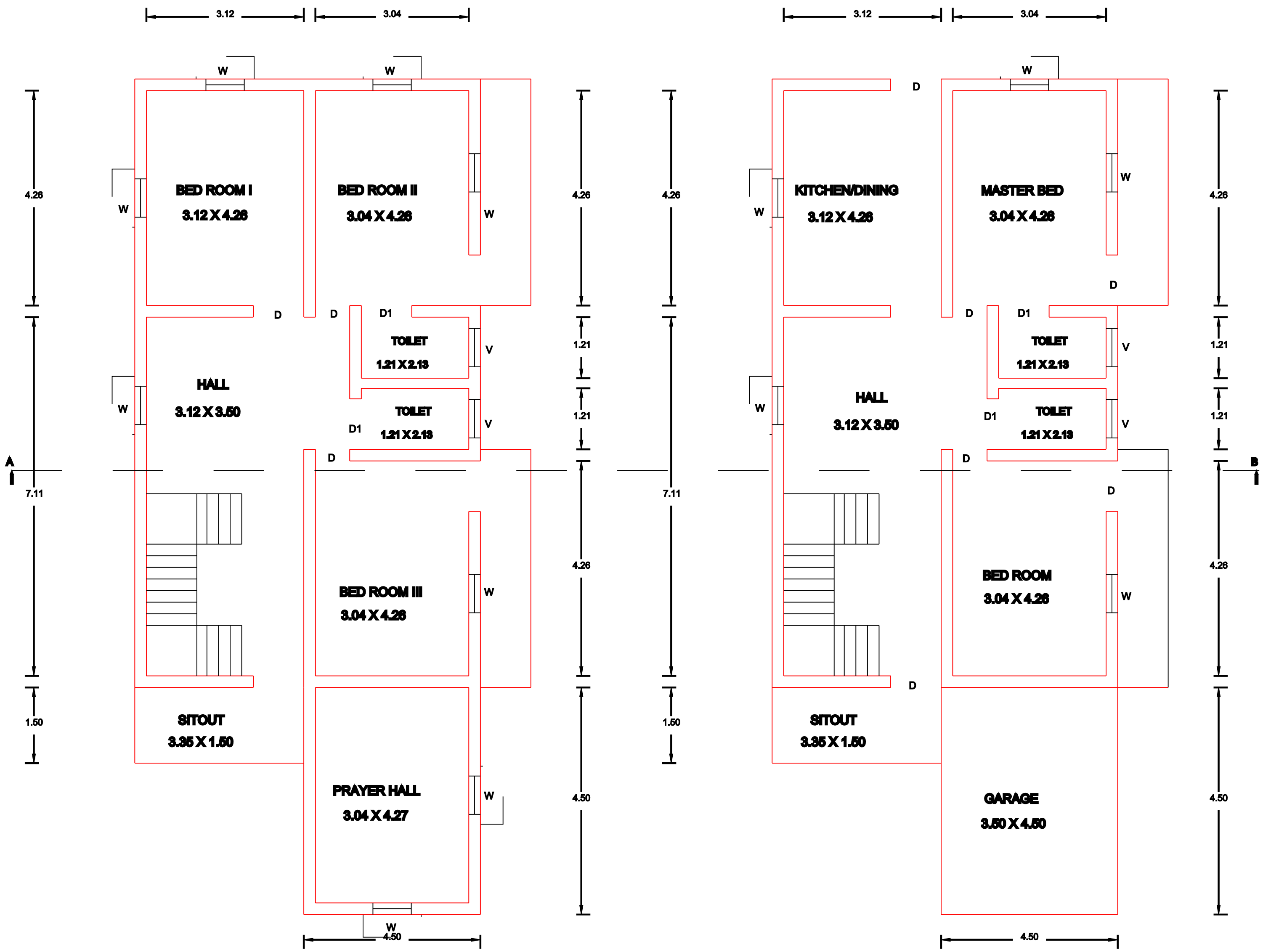
NORTH FACING
