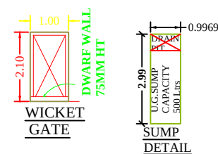
SUMP DETAIL
