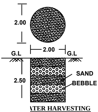
WATER HARVESTING
