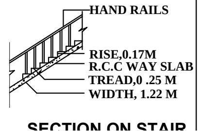
SECTION ON STAIR
