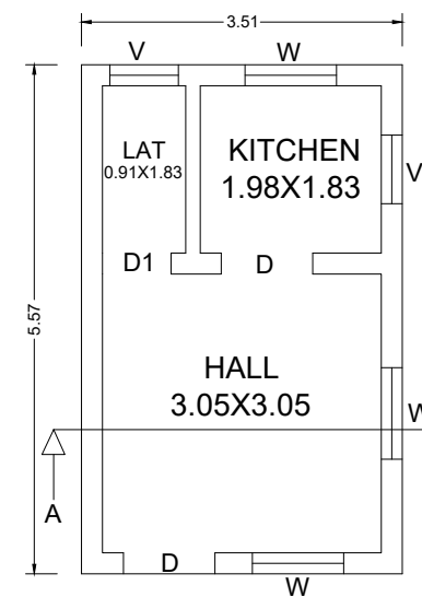
PLAN
