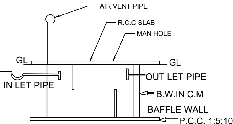
SECTION ON SEPTIC TANK
