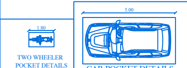
CAR POCKET DETAILS
