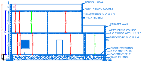
SECTION ON 'XX'
