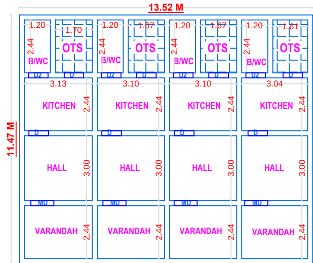
PLAN - GROUND FLOOR
