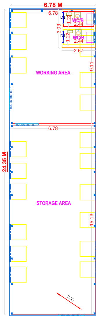
PLAN - GROUND FLOOR (PRO. COMMERCIAL BUILDING)
